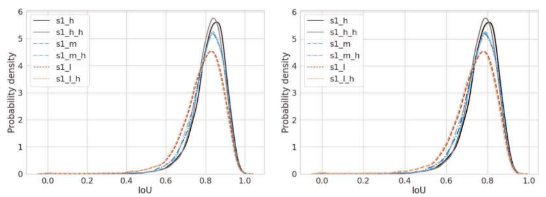
FIGURE 12 Distribution of intersection over union values for detection models, (left): day time; (right): night time [Color figure can be viewed at wileyonlinelibrary.com ]
