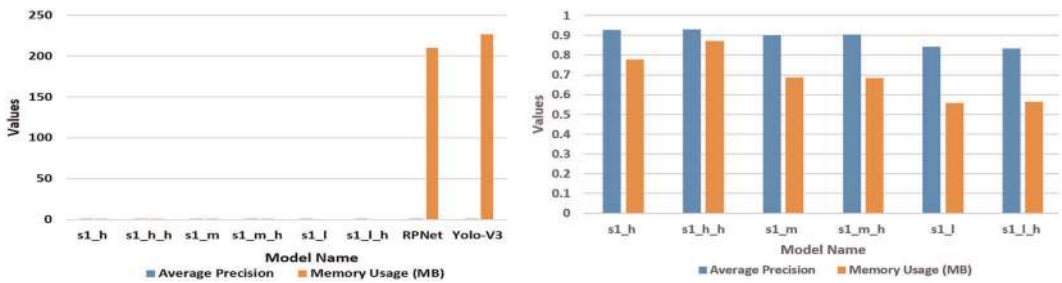
FIGURE 15 Detection model size vs average precision for daytime, (left): comparison with the existing models and (right): enlarged view of the model results [Color figure can be viewed at wileyonlinelibrary.com ]
