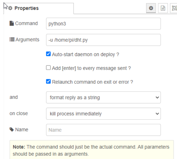
Figure 2.4: Configuring the daemon Node with python3 -u /home/pi/dht.py
