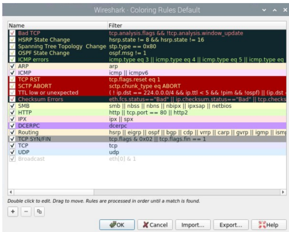
Figure 7.11: Editing Color Rules
