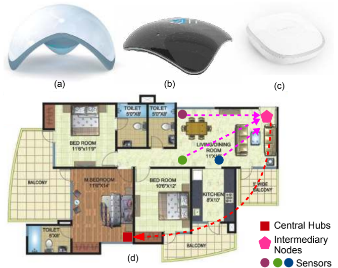
Fig. 15. Centralised Hubs are category of devices heavily used in IoT solution. (a) Ninja sphere (b) ALYT Hub powered by Andorid (c) Samsung's SmartThings Hub (d) Sensors and other components are connected to a centralised hub. These hubs are typically connected to permanent power sources and comprises comparatively high computational capabilities.
