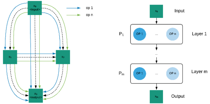
Figure 8. Stochastic super network (left): PC-DARTS, (right): FBNet.
