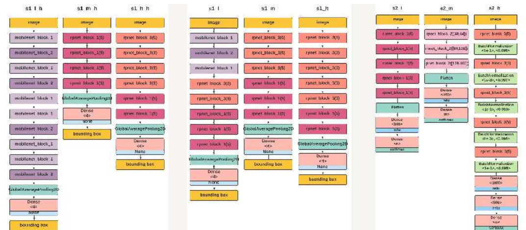
Figure 9. Model Architectures (left): hardware optimized detection, (middle): hardware agnostic detection, (right): recognition subnetworks.
