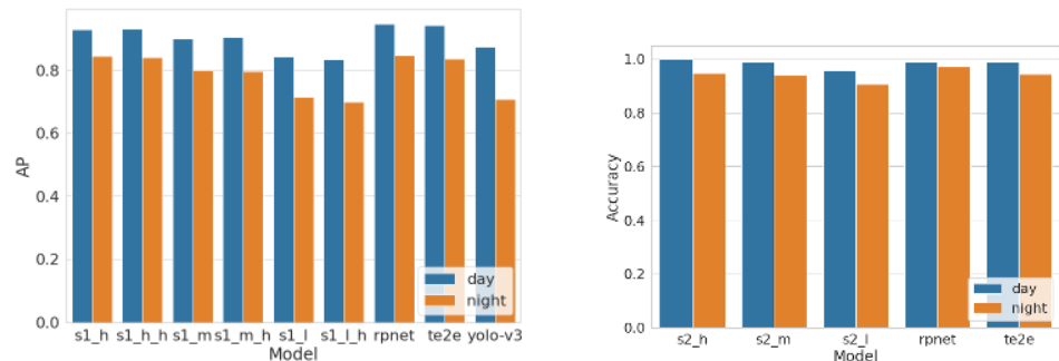
Figure 10. Model accuracy on the synthetically generated dataset (left): detection, (right) recognition.
