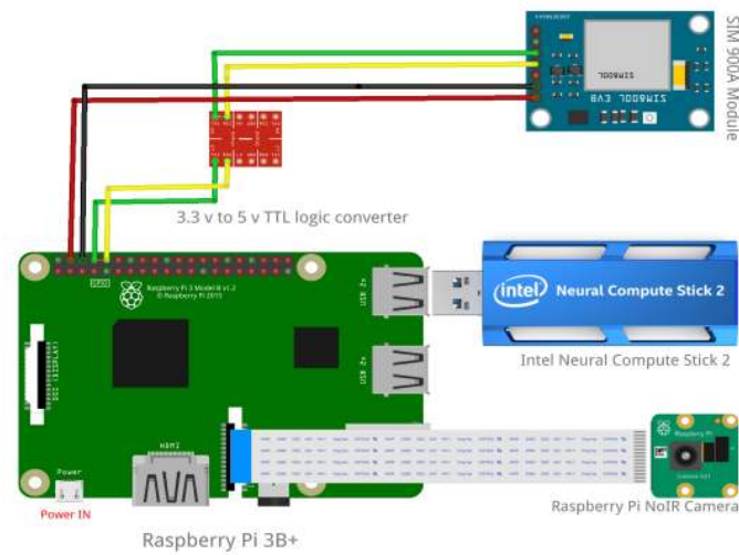
Figure 5. Circuit diagram of the design
