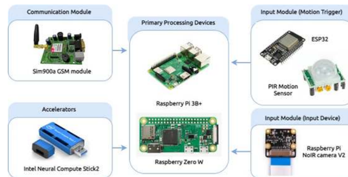
Figure 2. Hardware stack of the proposed solution
