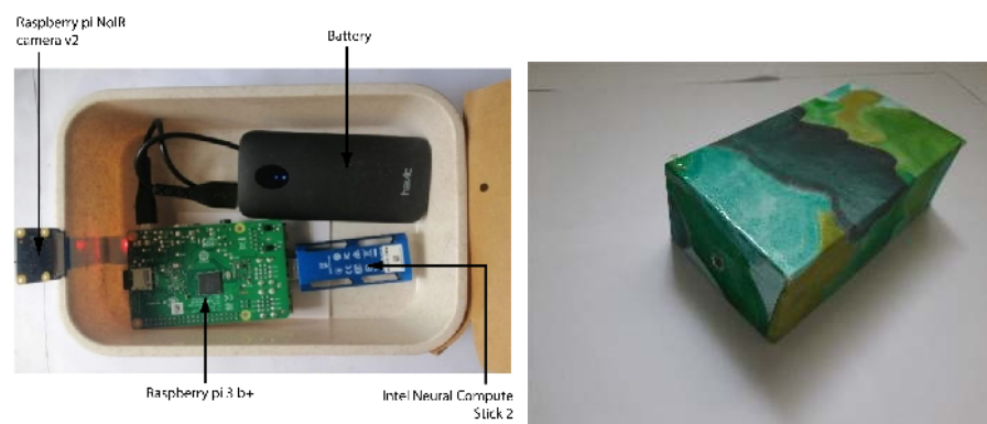
Figure 4. High-tier model (left): Internal view, (right): Exterior deployment view.
