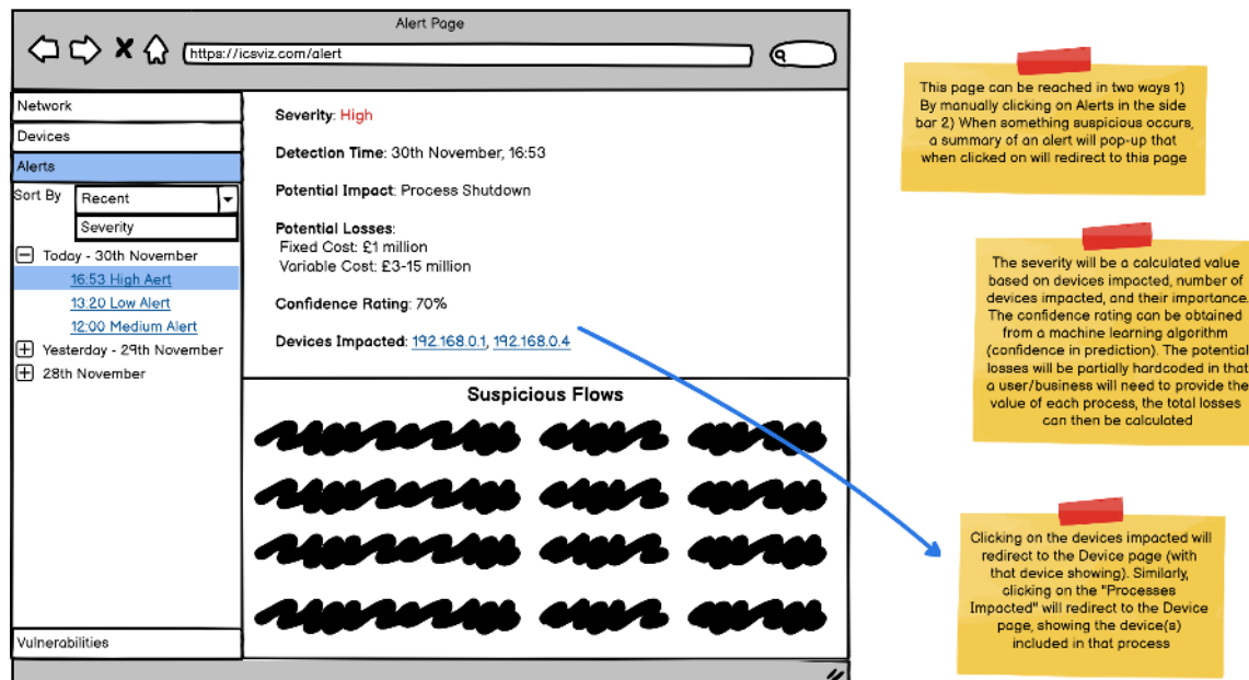
Figure 10. Alert Page
