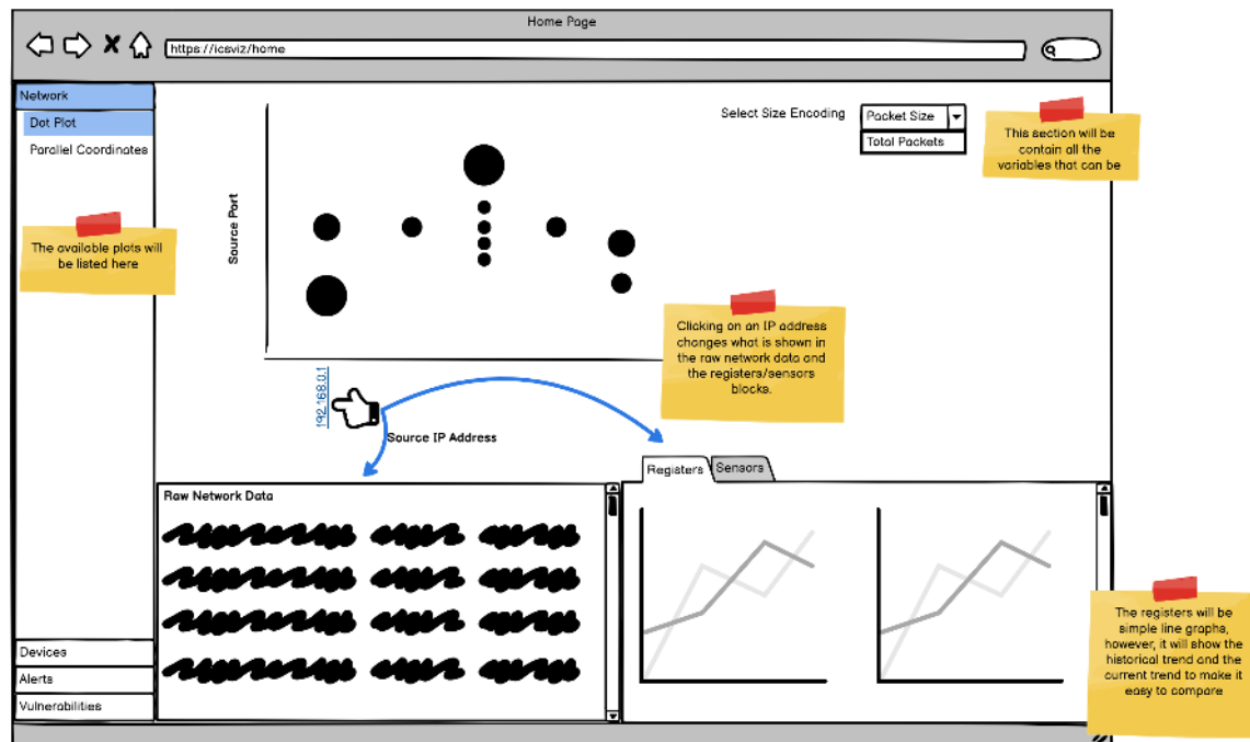
Figure 8. Overview Page
