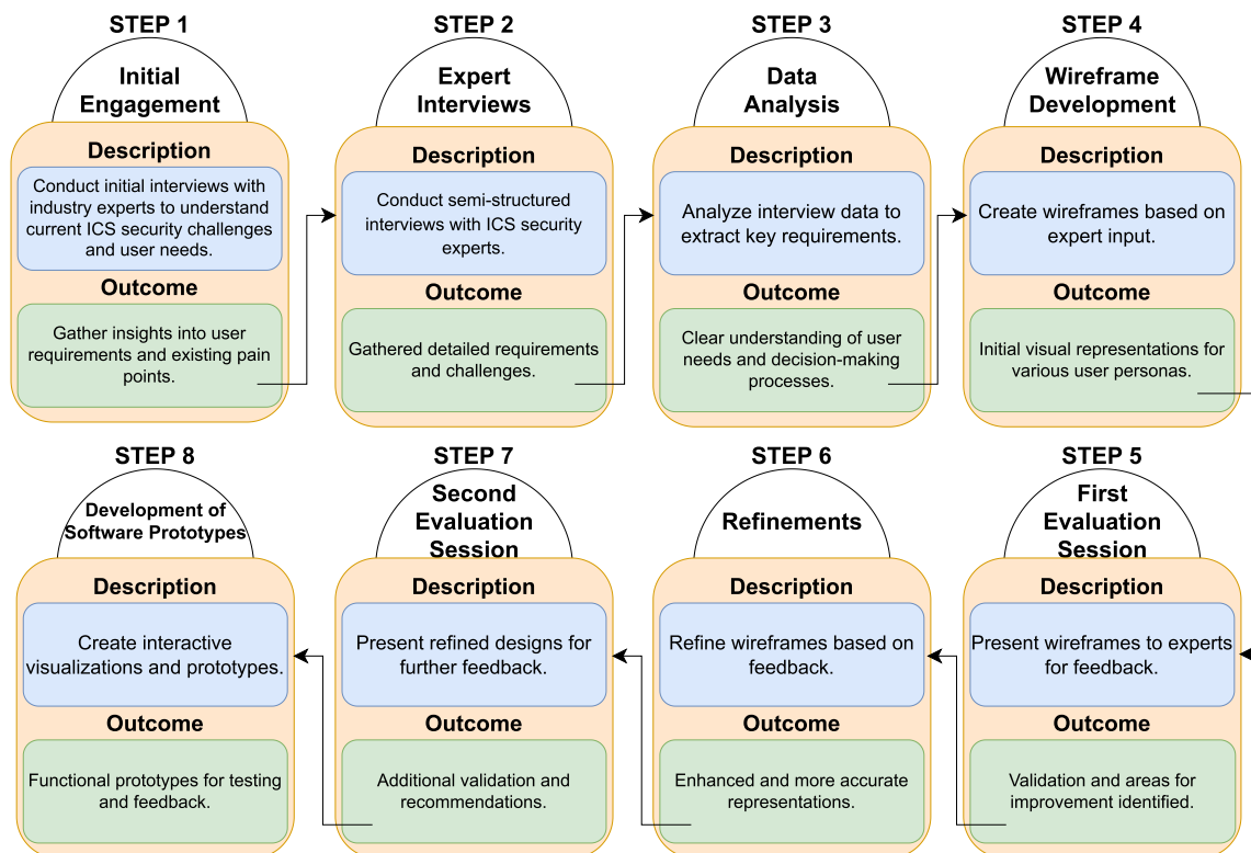
Figure 2. The methodology.
