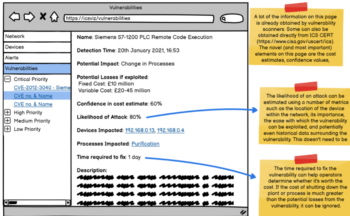
Figure 11. Vulnerabilities Page
