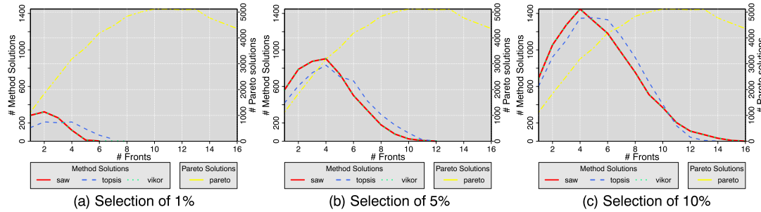
Figure 6. Pareto fronts for five context properties. SAW, simple additive weight; TOPSIS, technique for the order of prioritization by similarity to ideal solution; VIKOR, VlseKriterijumska Optimizacija I Kompromisno Resenje.
