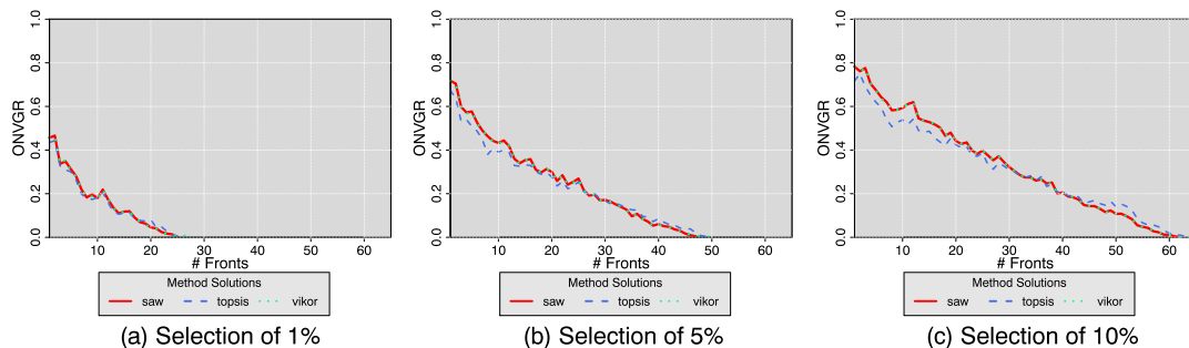
Figure 10. Overall non-dominated vector generation ratio (ONVGR) metric for three context properties. SAW, simple additive weight; TOPSIS, technique for the order of prioritization by similarity to ideal solution; VIKOR, VIseKriterijumska Optimizacija I Kompromisno Resenje.
