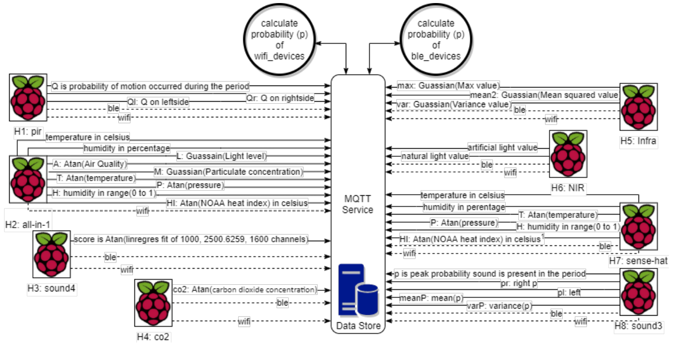
Fig. 1 H1: Passive InfraRed, H2: All-in-1 Multi-sensor, H3: Sound4, H4: Carbon Dioxide, H5: Infra-sound, H6: Light, H7: Sense-Hat Multi-sensor, H8: Sound3
