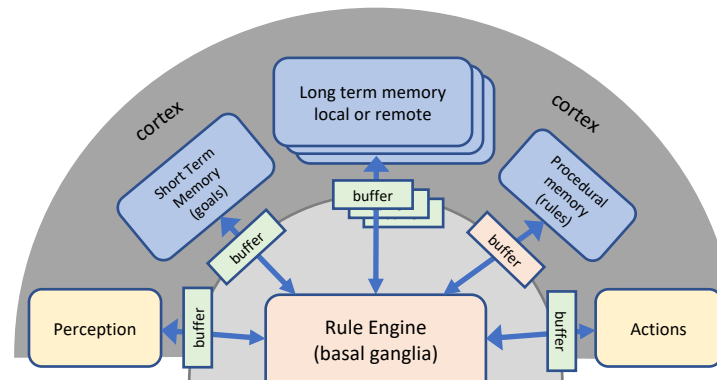
Cognition – Sequential Rule Engine
