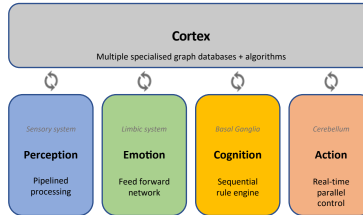
Cognitive Architecture with multiple cognitive circuits loosely equivalent to shared blackboard
